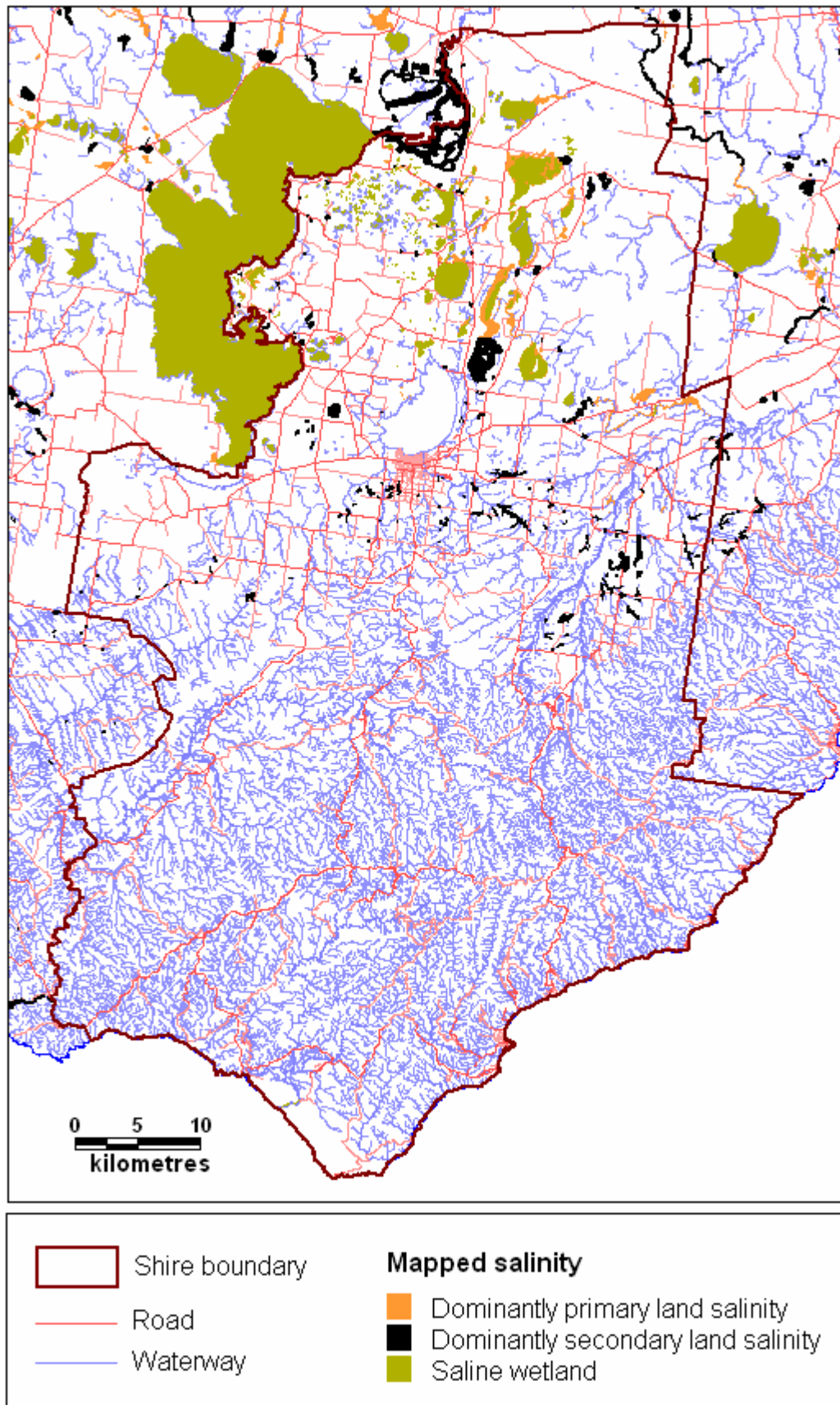
Figure 3.1 Salinity distribution in the Colac Otway Shire
