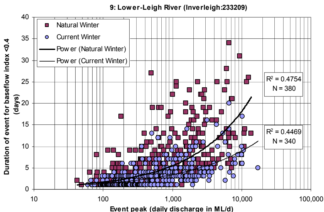
Figure 41. Duration of Winter flood events for Lower Leigh River. Discharge is peak event discharge (measured as daily flow).
