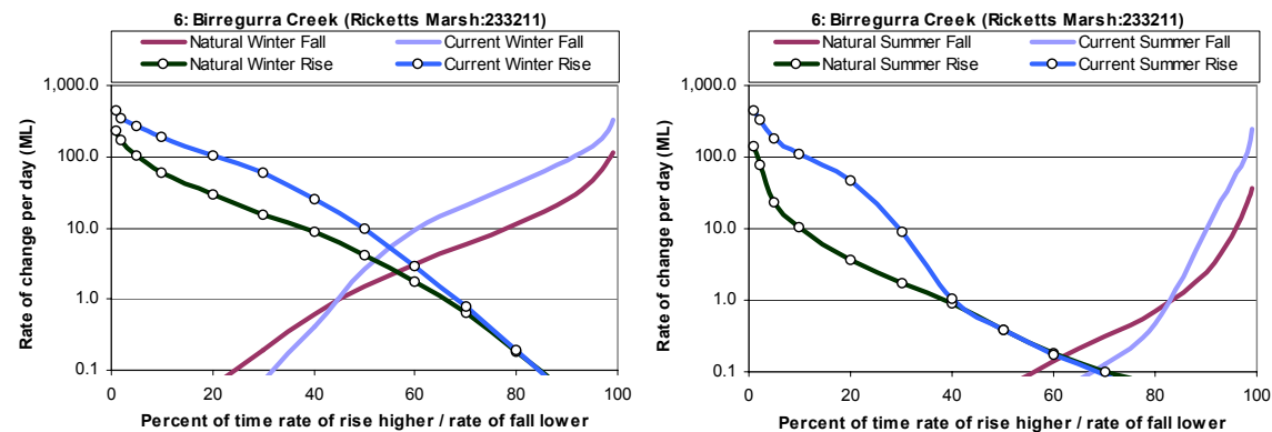
Figure 49. Distribution of natural and current daily changes in discharge (rise and fall) for stormflow, Birregurra Creek.
