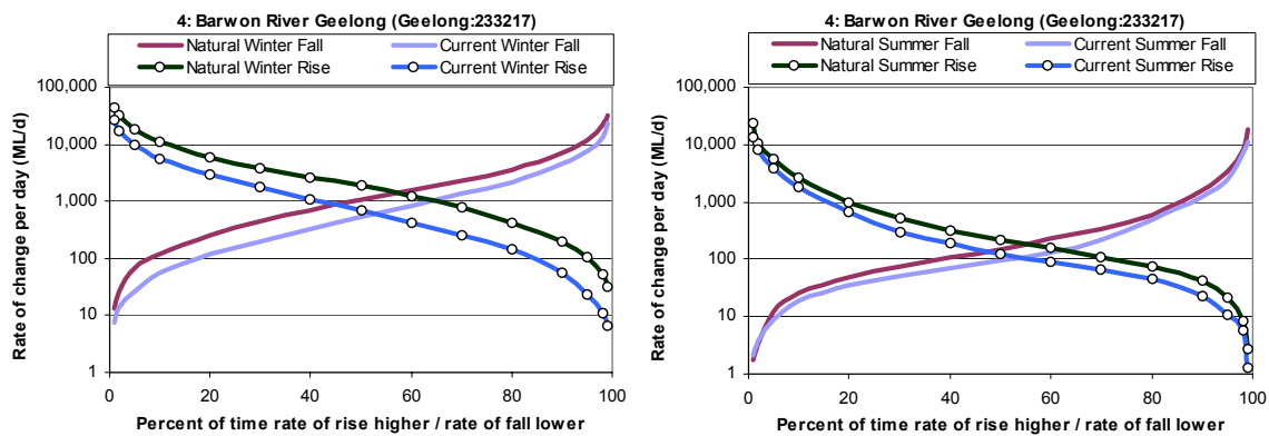
Figure 48. Distribution of natural and current daily changes in discharge (rise and fall) for stormflow, Barwon River Geelong.
