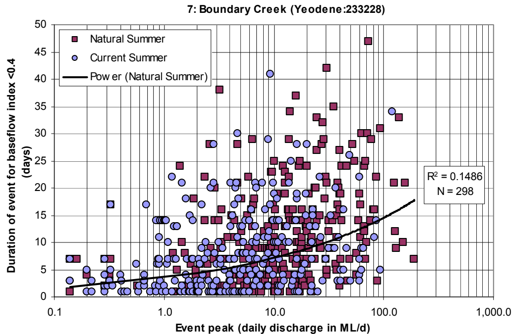
Figure 25. Duration of Summer flood events for Boundary Creek. Discharge is peak event discharge (measured as daily flow).
