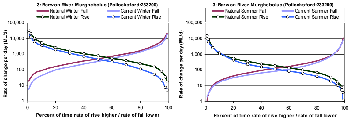
Figure 47. Distribution of natural and current daily changes in discharge (rise and fall) for stormflow, Barwon River Murgheboluc.
