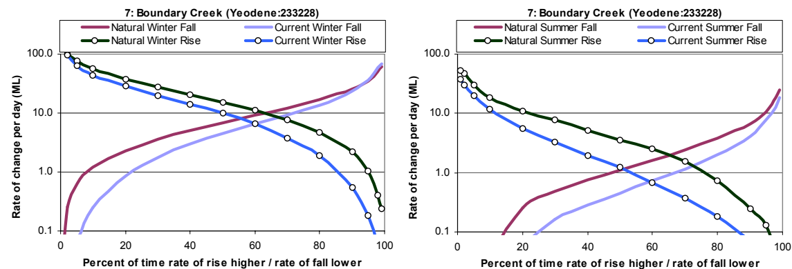
Figure 50. Distribution of natural and current daily changes in discharge (rise and fall) for stormflow, Boundary Creek.
